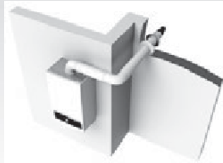
Figure A.3.2 Maximum Equivalent Flue Length 6 m
