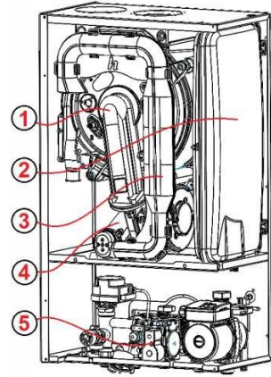
Figure 1.4.2: Main component
