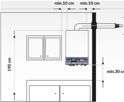
Figure 1.2.2: Mounting Place
