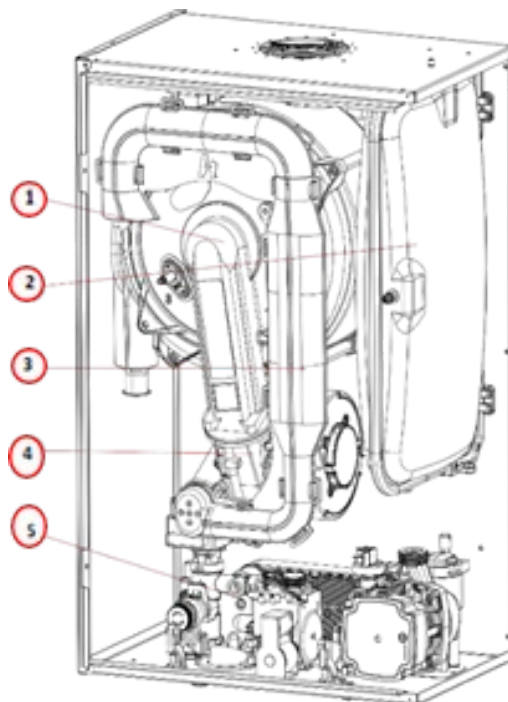
Figure 4. 2 Device introduction
